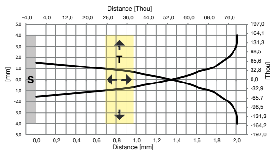
Fig. 3 Non-flush, 2mm
