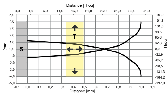
Fig. 1 Flush, 1mm
