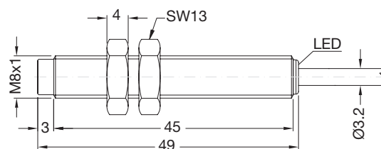
Fig. 15 Long body, non-flush version, cable
